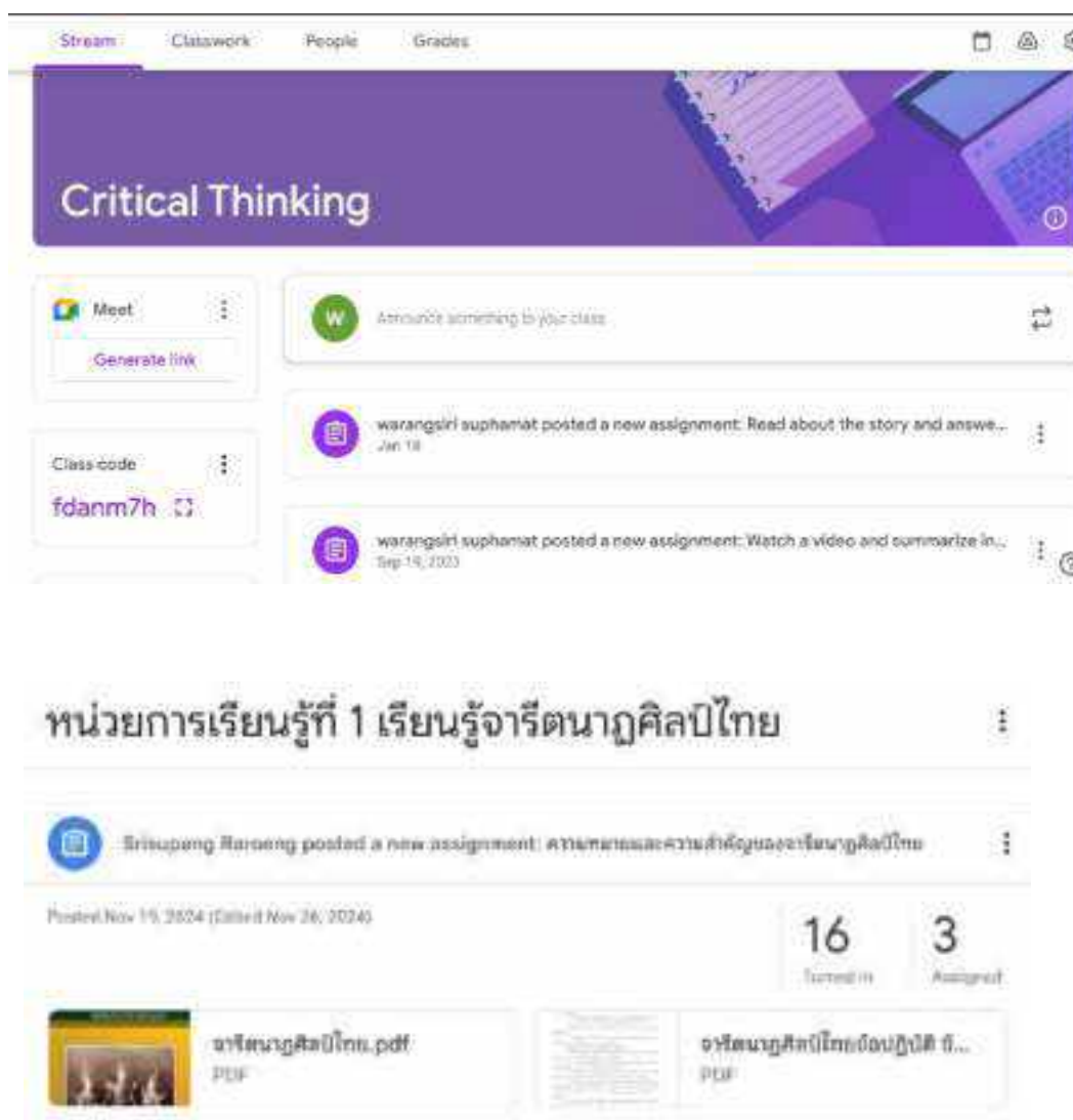
Google Classroom
