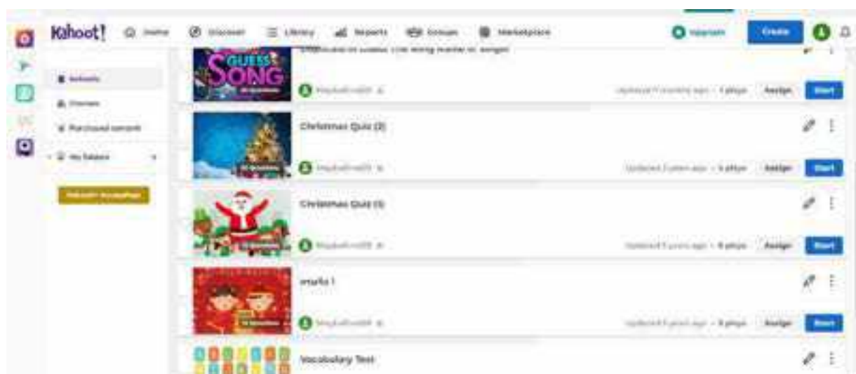
Kahoot
